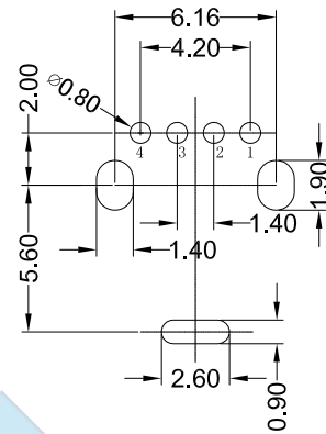
PCB LAYOUT MOUNTING PATTERN
