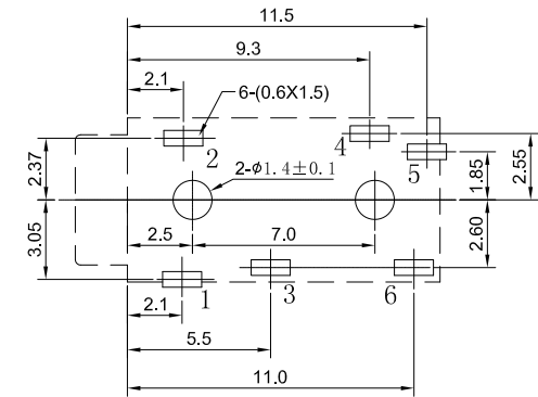
P.C.B LAYOUT MOUNTING PATTERN (TOP VIEW)
