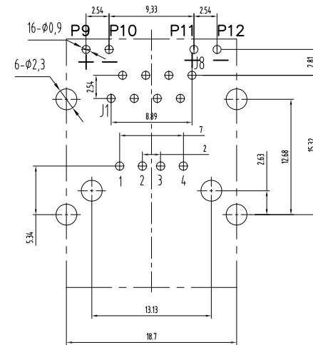
RECOMMEND PCB LAYOUT
