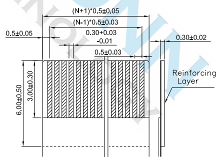
RECOMMENDED FFC/FPC DIM.
