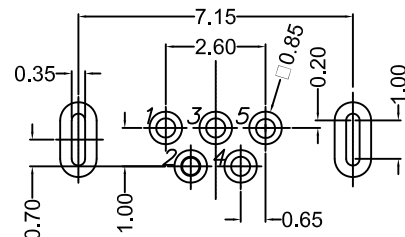
PCB LAYOUT MOUNTING PATTERN
