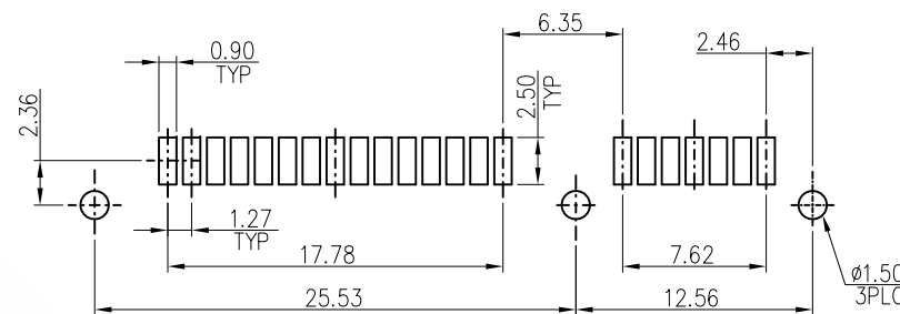
P C B Layout PCB TOLERANCE: ±0.05
