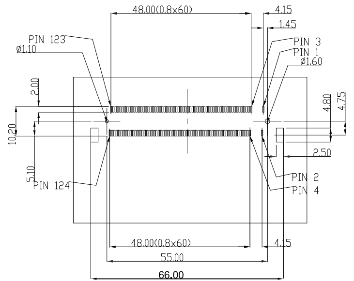
RECOMMEND PC BOARD LAYOUT
