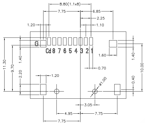
RECOMMEND PC BOARD LAYOUT
