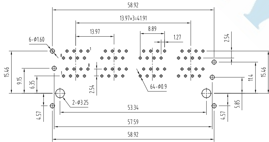
PCB LAYOUT
