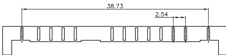
RECOMMENDED PCB LAYOUT PCB TOLERANCE:±0.05
