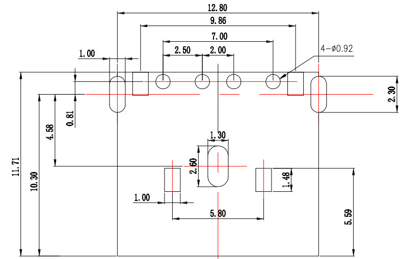
RECOMMENDED P.C.B.LAYOUT
