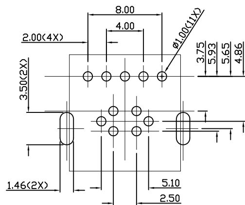
PCB LAYOUT
