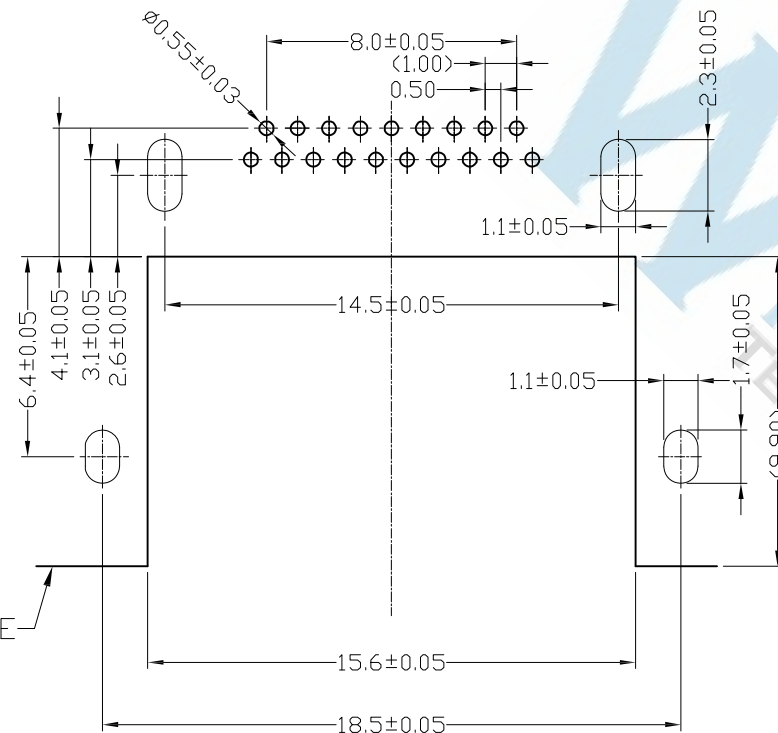
RECOMMENDED PCB LAYOUT (THICKNESS=1.2±0.10mm)
