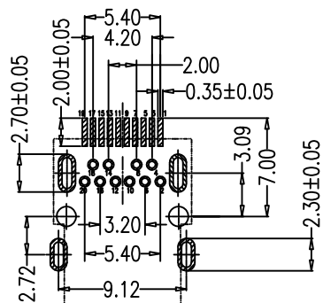
P.C.B Layout t=1.60mm Component side
