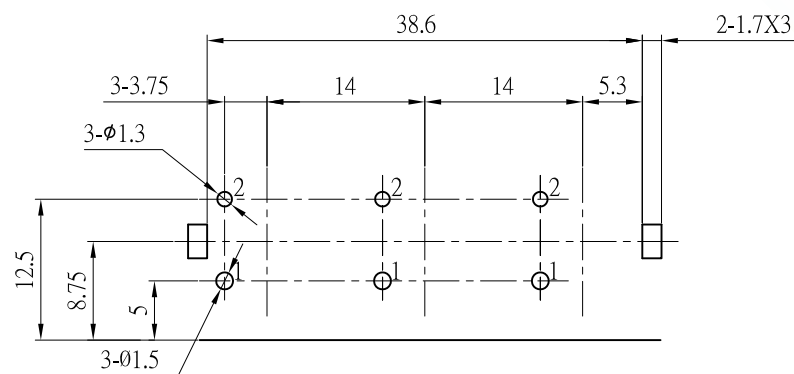
PCB Holes Diagram Top View
