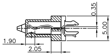
SECT B-B
